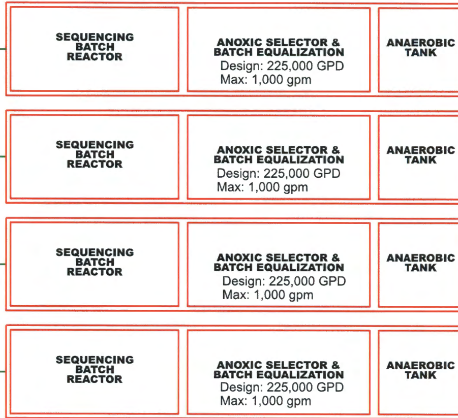
FIG 2-1 PROPOSED 0.9 MGD OWENS CROSS ROADS WWTP PROCESS FLOW DIAGRAM SNEAD AVENUE OWENS CROSS ROADS, AL 35763
