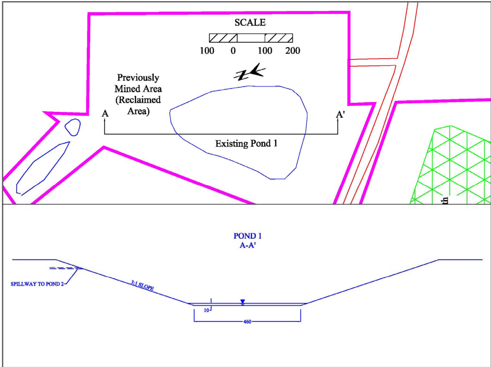
Figure 3: Pond 1 Cross Section and Plan View
