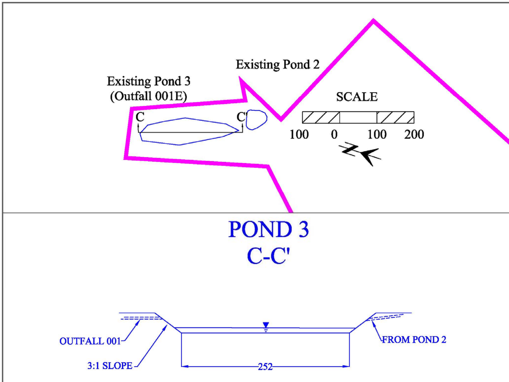
Figure 5: Pond 3 Cross Section and Plan View
