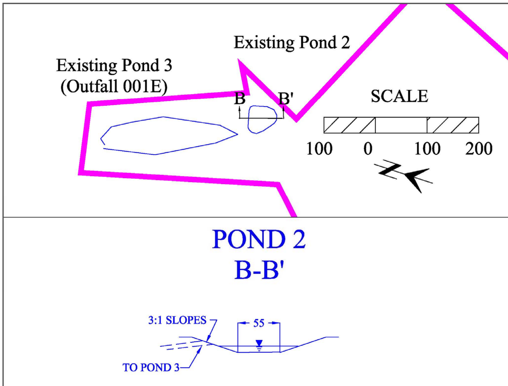
Figure 4: Pond 2 Cross Section and Plan View
