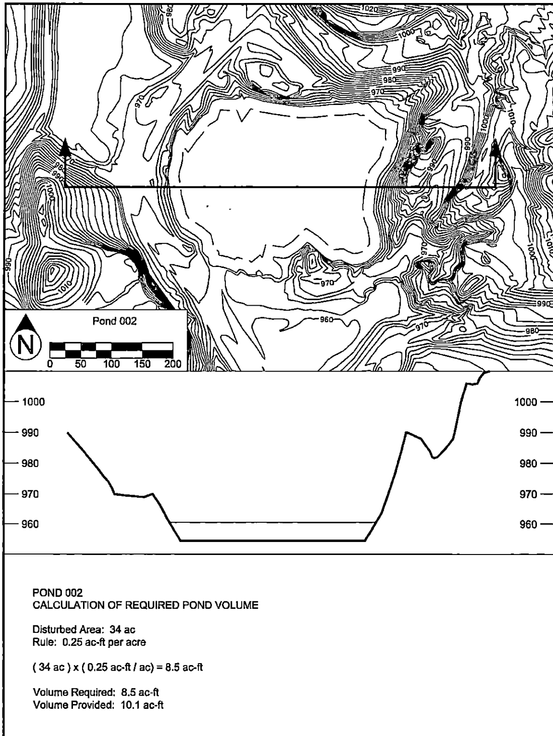
Figure 3-3. Pond 002.
