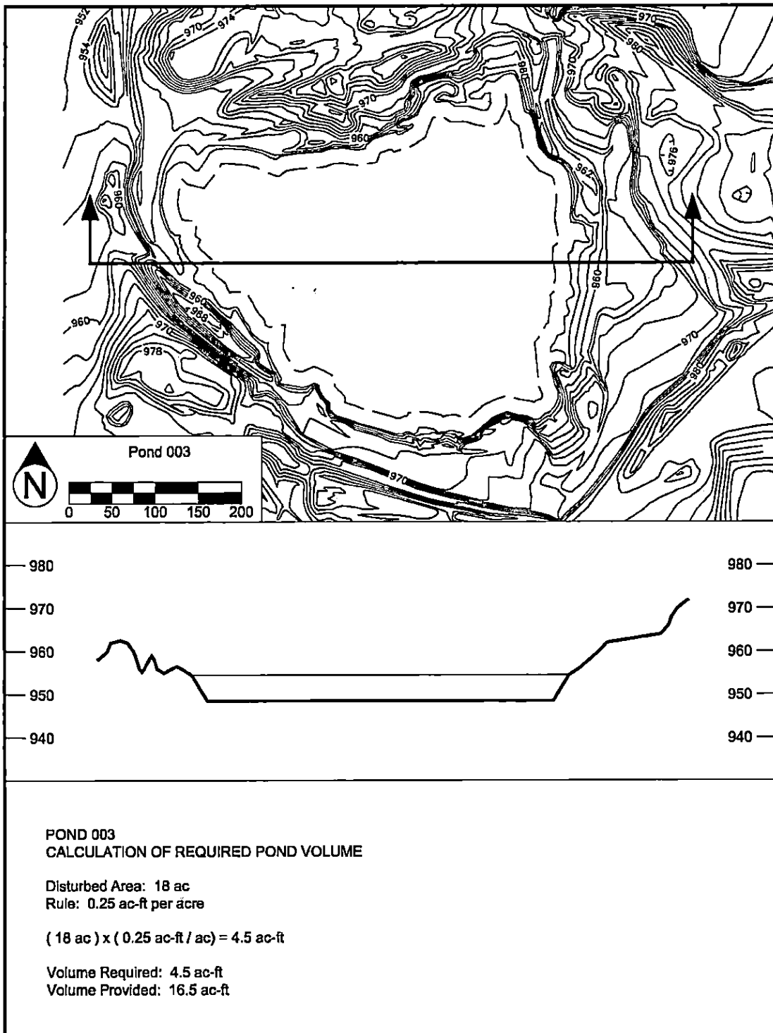
Figure 3-5. Pond 003.
