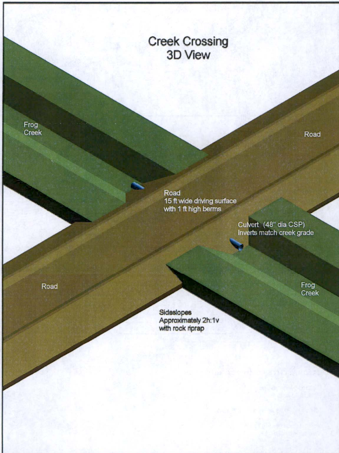
Figure 3-2. Creek Crossing.
