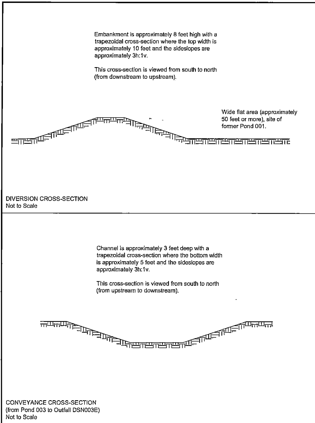
Figure 3-1. Cross-Sections.
