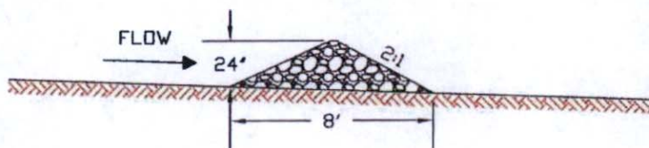
SECTION VIEW
