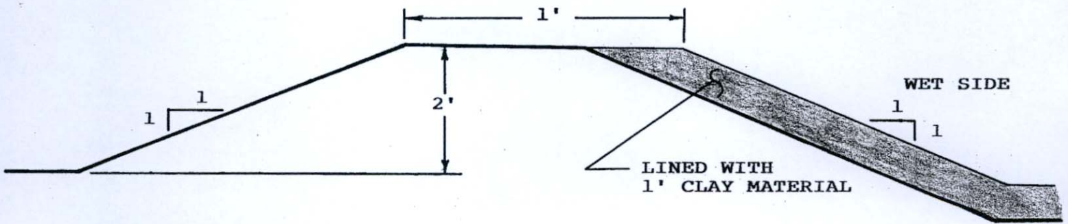
SIDE VIEW
